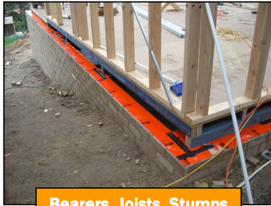
Bearers, Joists, Stumps
