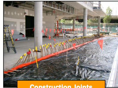
Construction Joints
